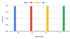
2 Qubits with Error Correction - Noisy Simulator
