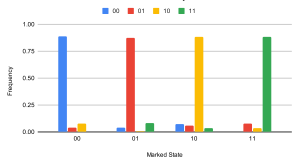
2 Qubits without Error Correction - Noisy Simulator
