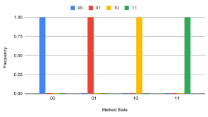
2 Qubits without Error Correction - Noiseless
