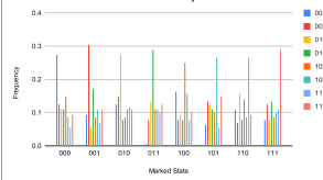
3 Qubits with Error Correction - Noisy
