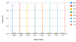
3 Qubits without Error Correction - Noiseless
