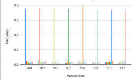
3 Qubits without Error Correction - Noisy Simulator
