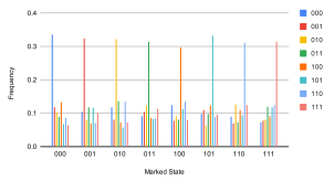
3 Qubits with Error Correction - Noiseless
