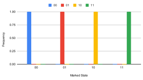
2 Qubits with Error Correction - Noiseless
